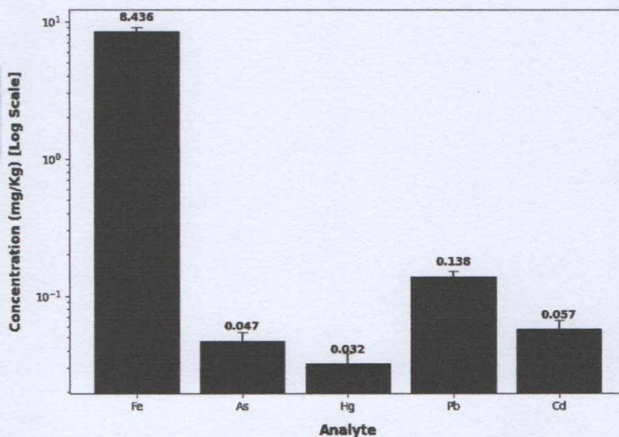
Haldi Sample: Analyte Concentrations with Standard Deviation
